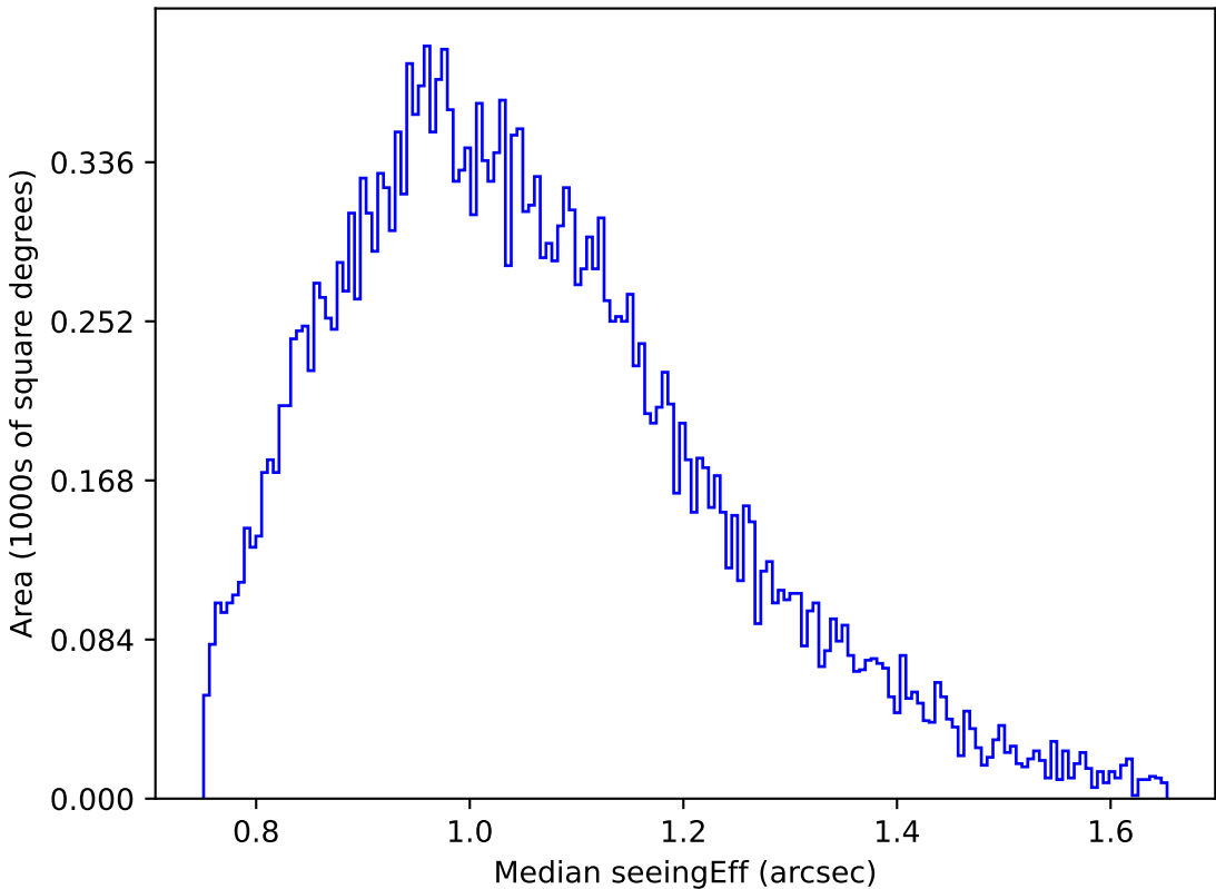
ddf_loaded_half_fl15_v3.4_10yrs Yr 1 g band: Median seeingEff
