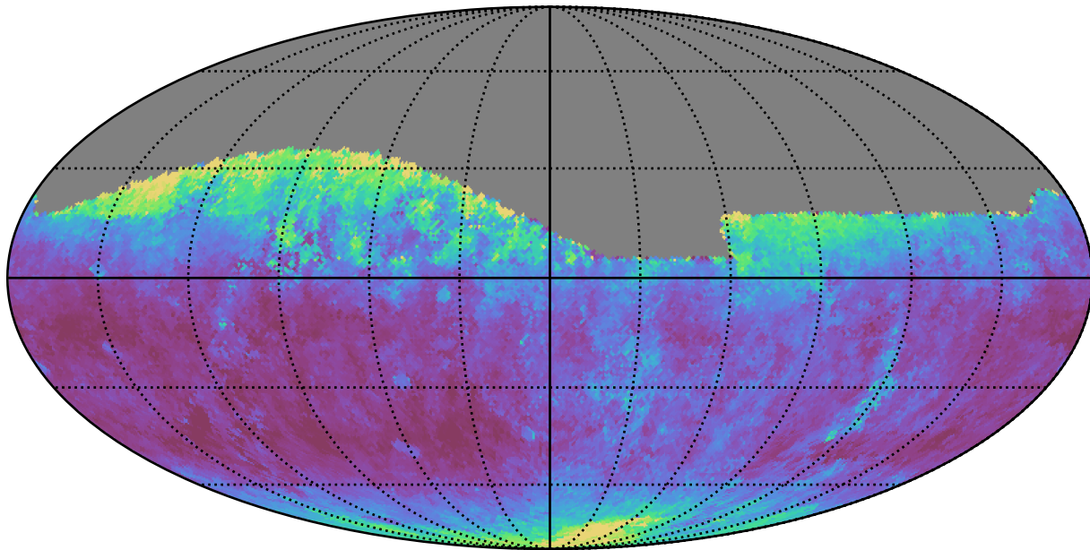
ddf_loaded_half_fl15_v3.4_10yrs Yr 1 all bands: Median seeingEff
