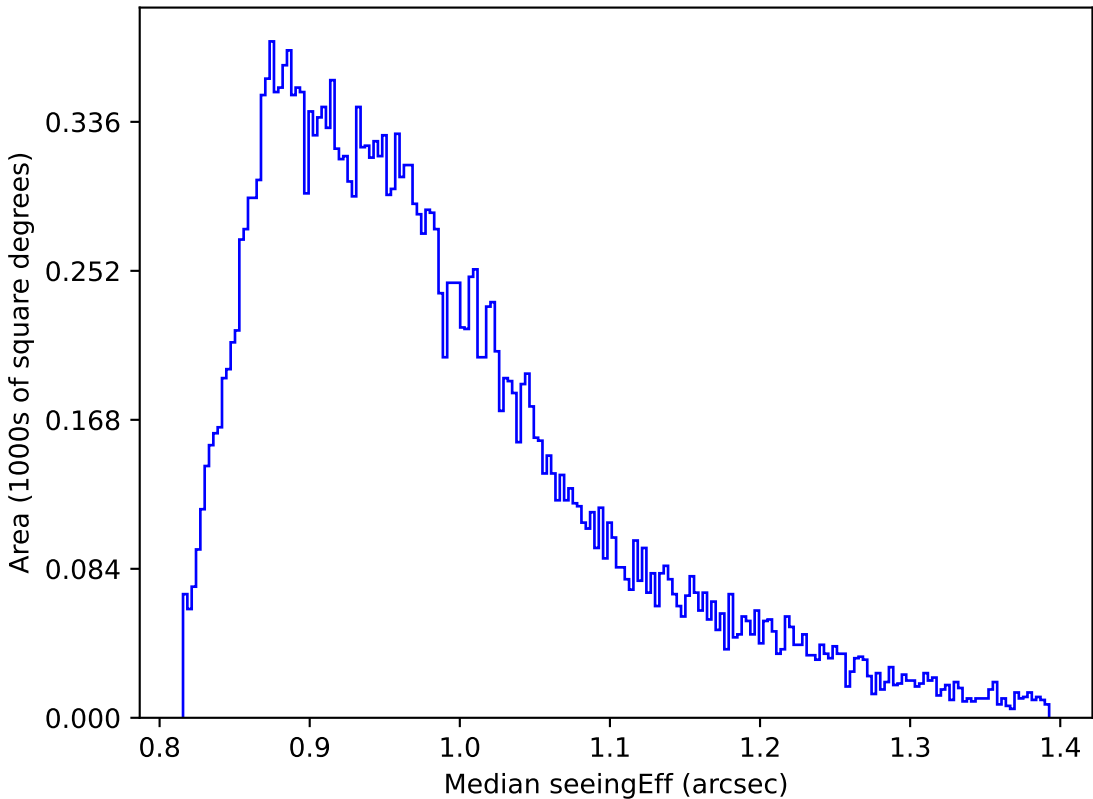
ddf_loaded_half_fl15_v3.4_10yrs Yr 1 all bands: Median seeingEff
