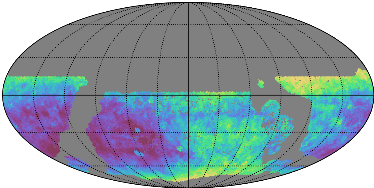
ddf_loaded_half_fl15_v3.4_10yrs WFD z band: Median seeingEff
