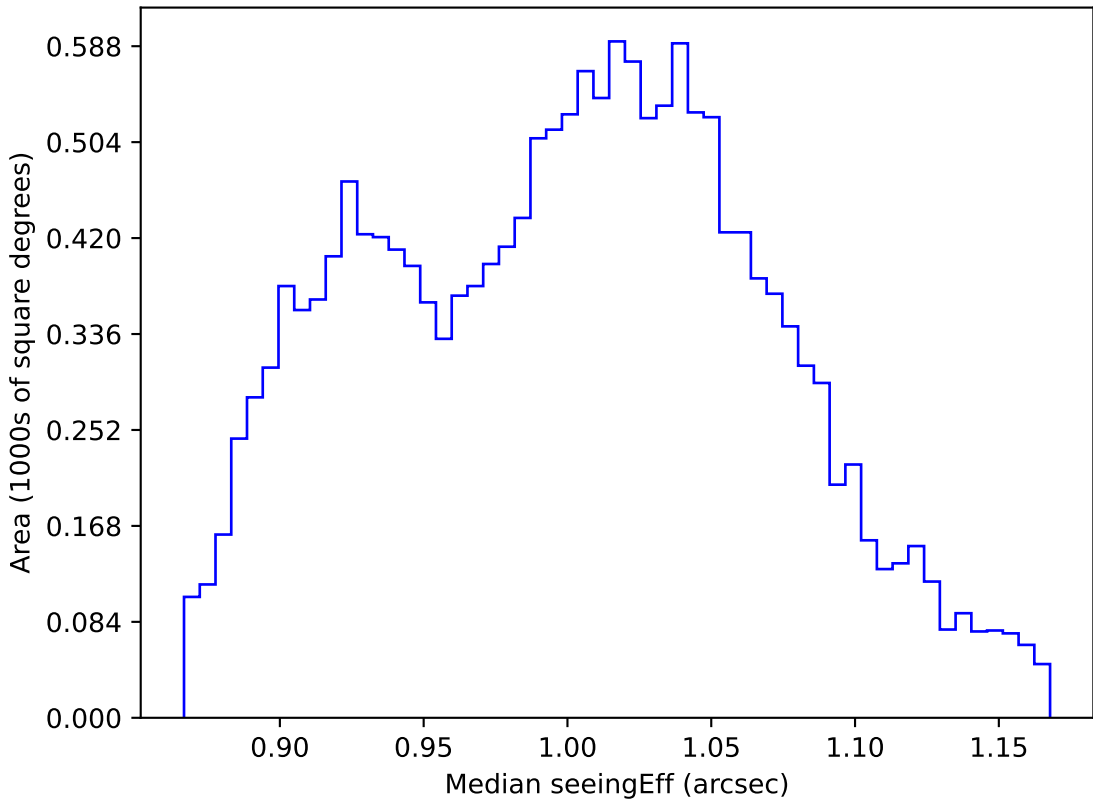
ddf_loaded_half_fl15_v3.4_10yrs WFD z band: Median seeingEff
