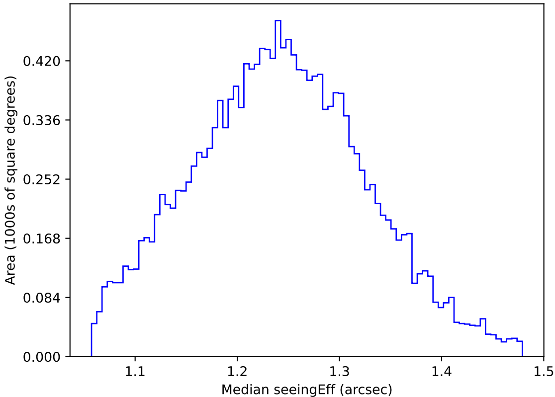
ddf_loaded_half_fl15_v3.4_10yrs WFD u band: Median seeingEff
