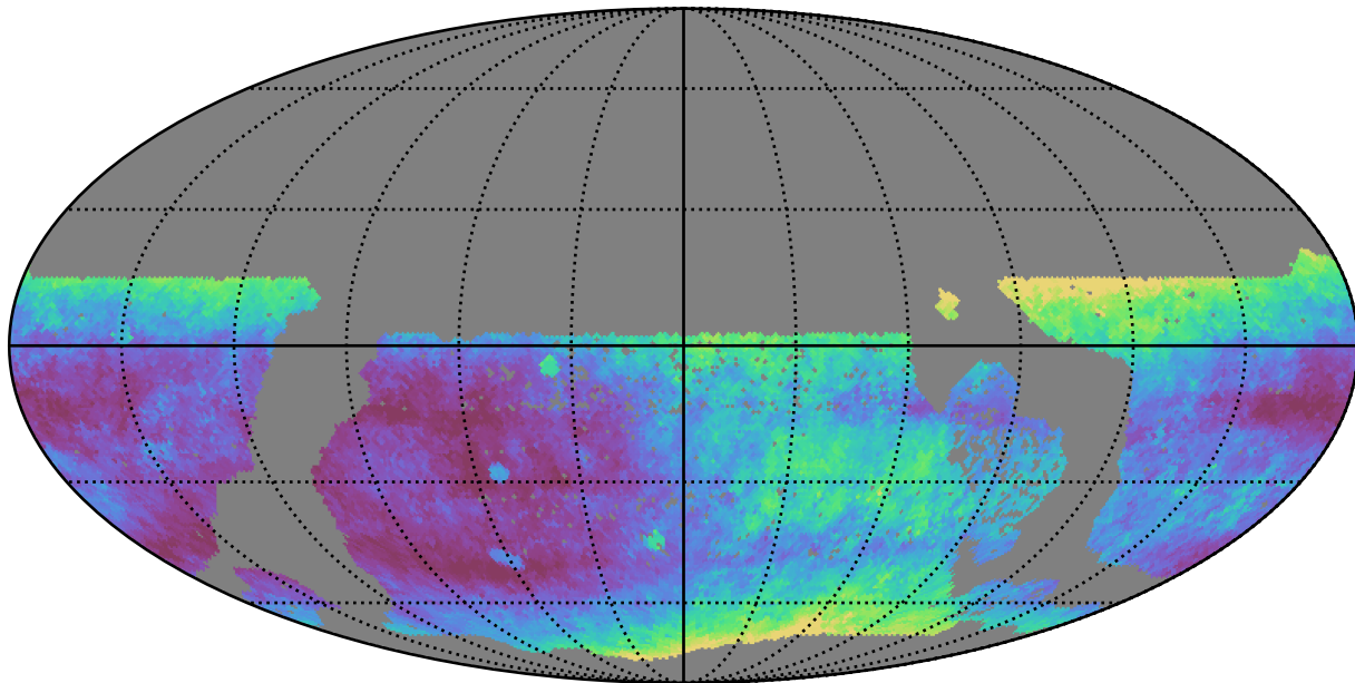
ddf_loaded_half_fl15_v3.4_10yrs WFD r band: Median seeingEff
