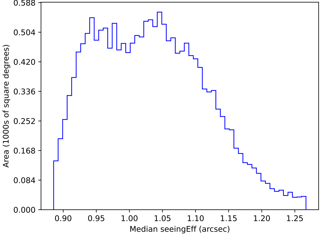
ddf_loaded_half_fl15_v3.4_10yrs WFD r band: Median seeingEff
