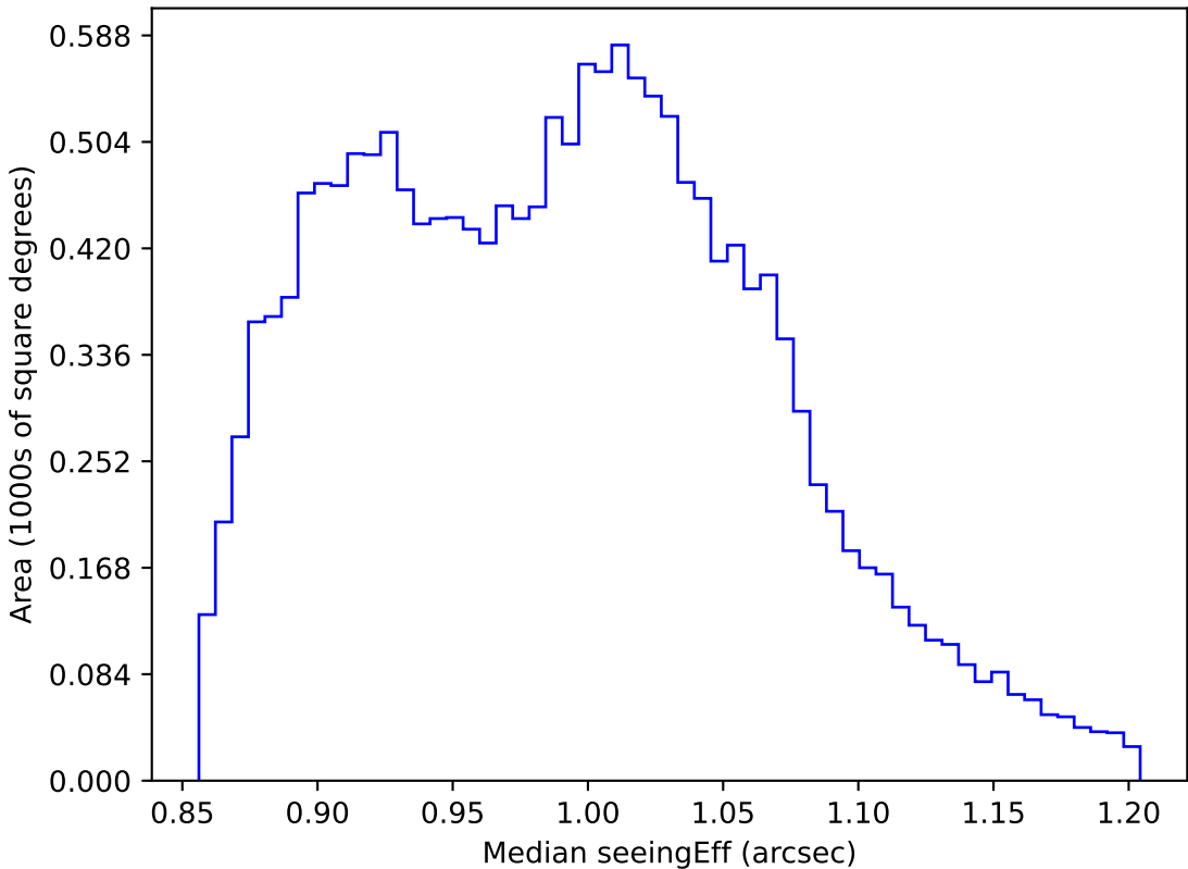
ddf_loaded_half_fl15_v3.4_10yrs WFD i band: Median seeingEff
