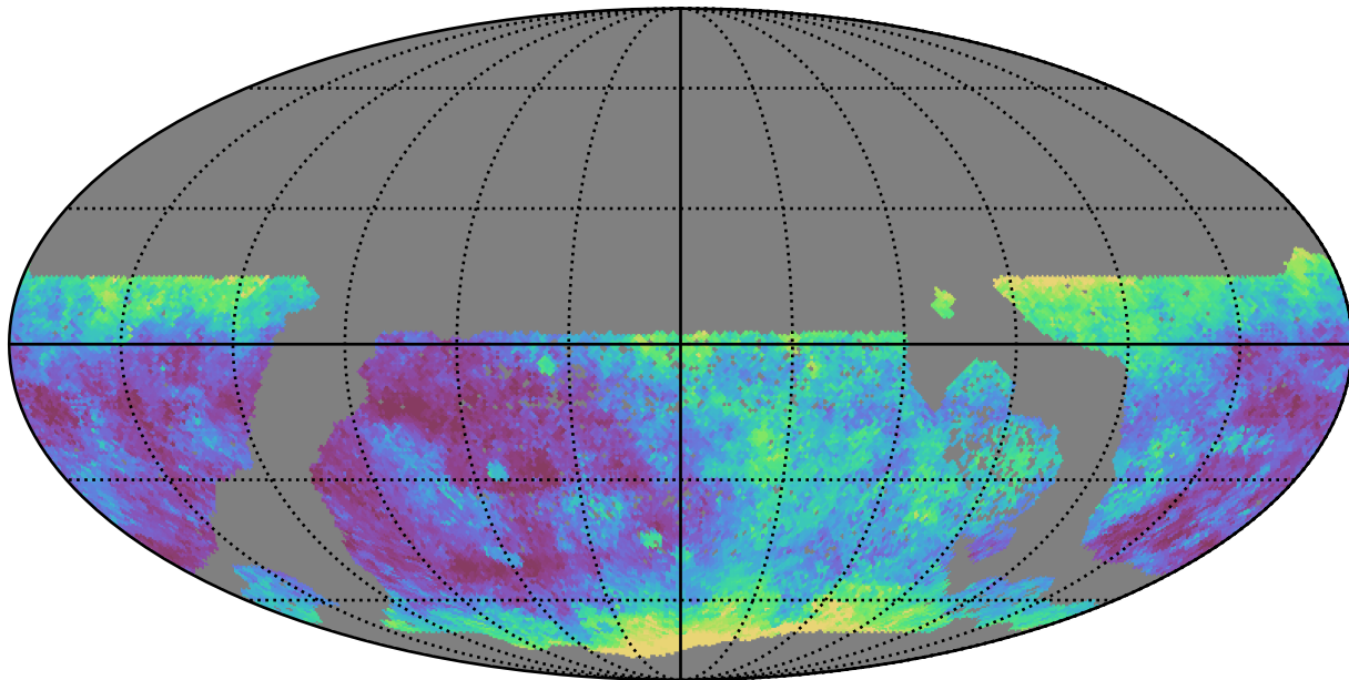
ddf_loaded_half_fl15_v3.4_10yrs WFD g band: Median seeingEff
