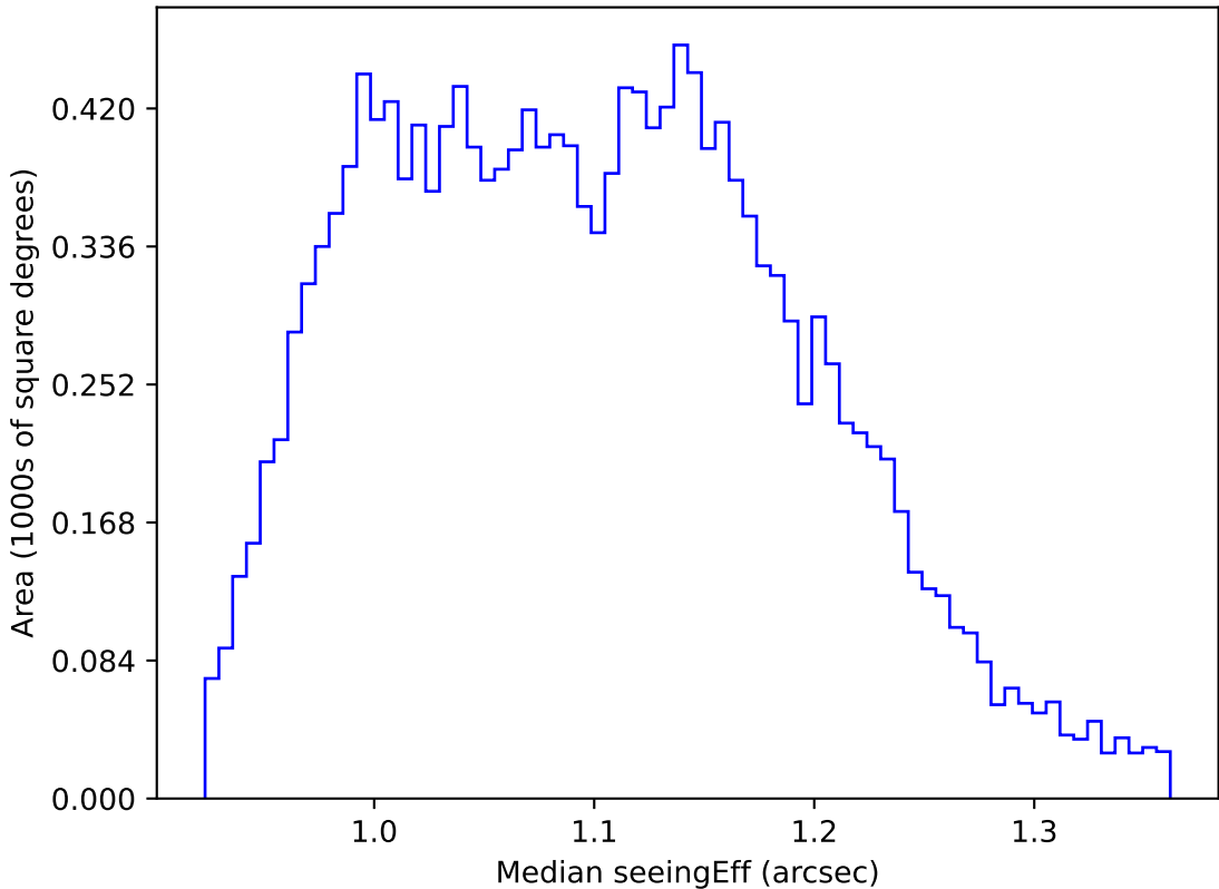
ddf_loaded_half_fl15_v3.4_10yrs WFD g band: Median seeingEff
