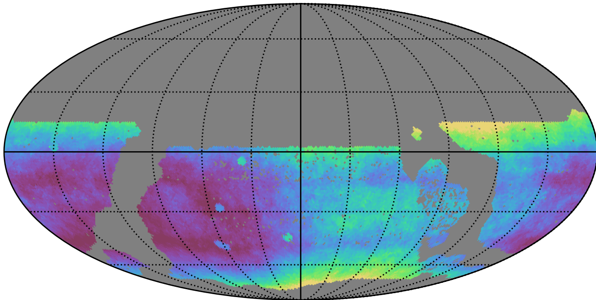
ddf_loaded_half_fl15_v3.4_10yrs WFD all bands: Median seeingEff
