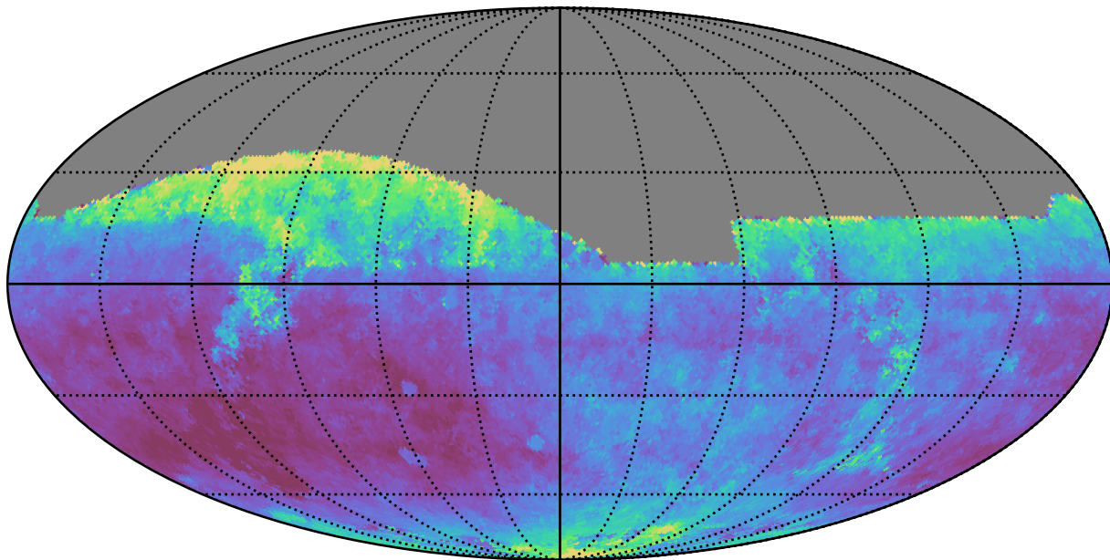
ddf_loaded_half_fl15_v3.4_10yrs All sky z band: Median seeingEff
