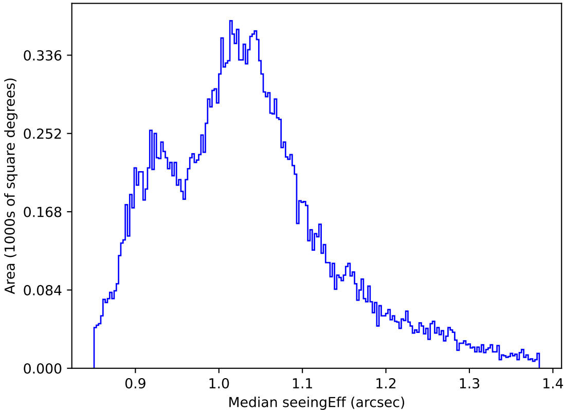
ddf_loaded_half_fl15_v3.4_10yrs All sky z band: Median seeingEff
