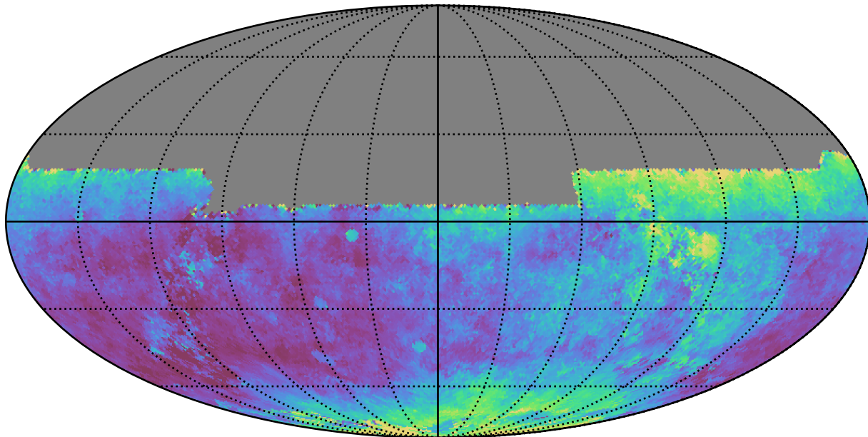
ddf_loaded_half_fl15_v3.4_10yrs All sky y band: Median seeingEff
