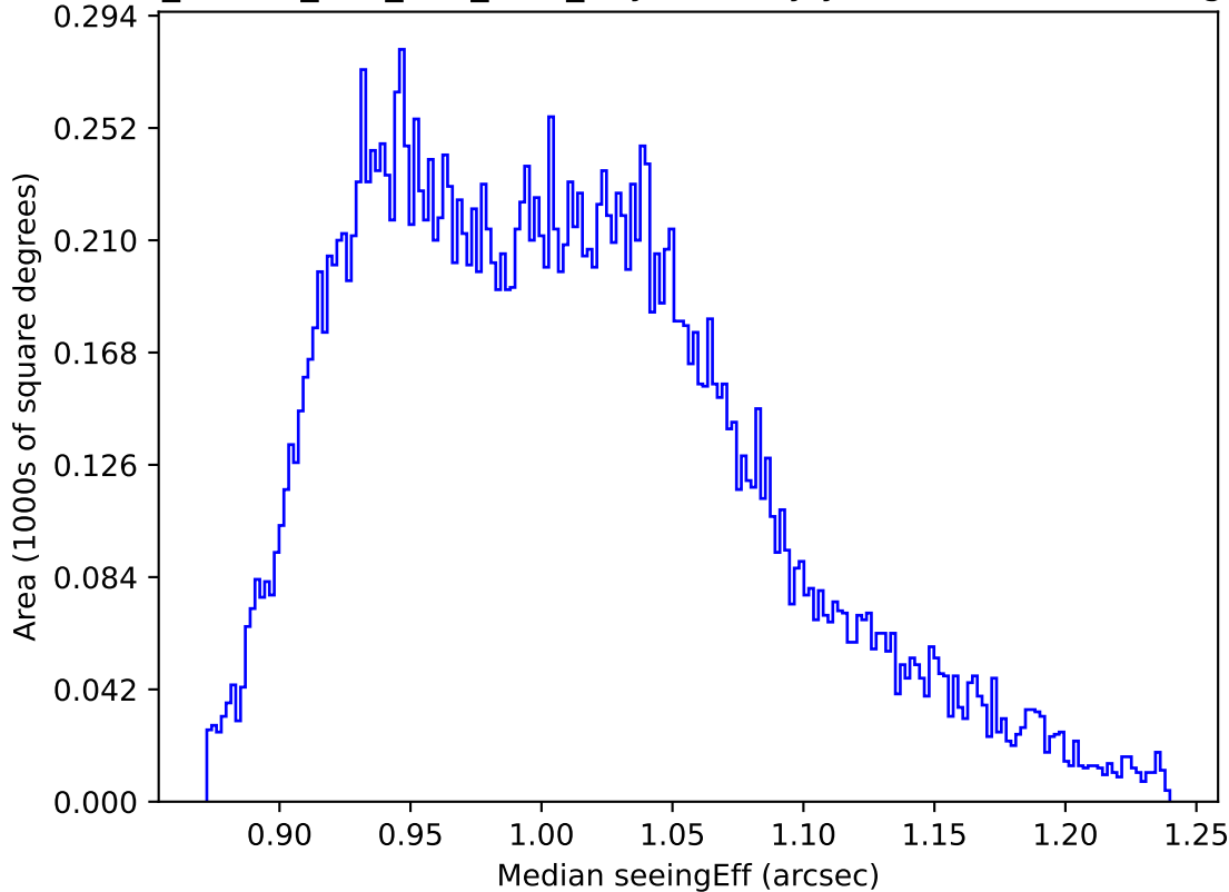
ddf_loaded_half_fl15_v3.4_10yrs All sky y band: Median seeingEff
