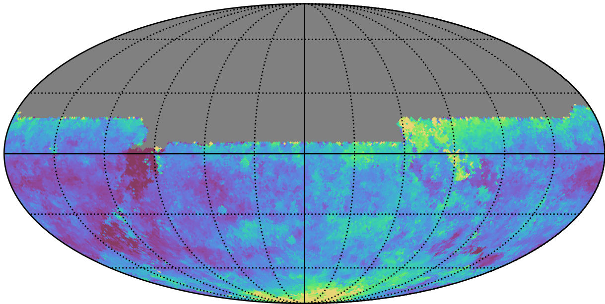
ddf_loaded_half_fl15_v3.4_10yrs All sky u band: Median seeingEff
