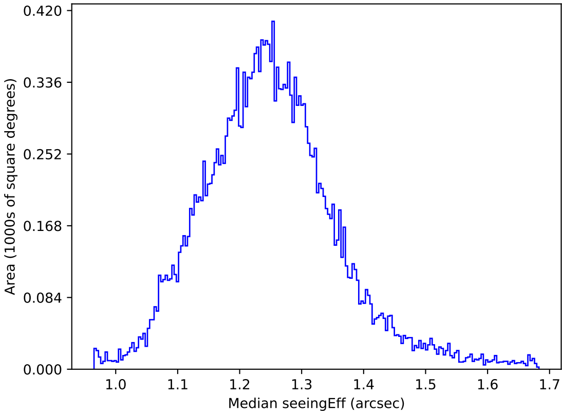
ddf_loaded_half_fl15_v3.4_10yrs All sky u band: Median seeingEff
