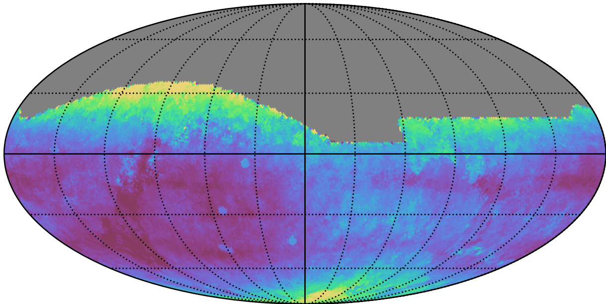
ddf_loaded_half_fl15_v3.4_10yrs All sky r band: Median seeingEff
