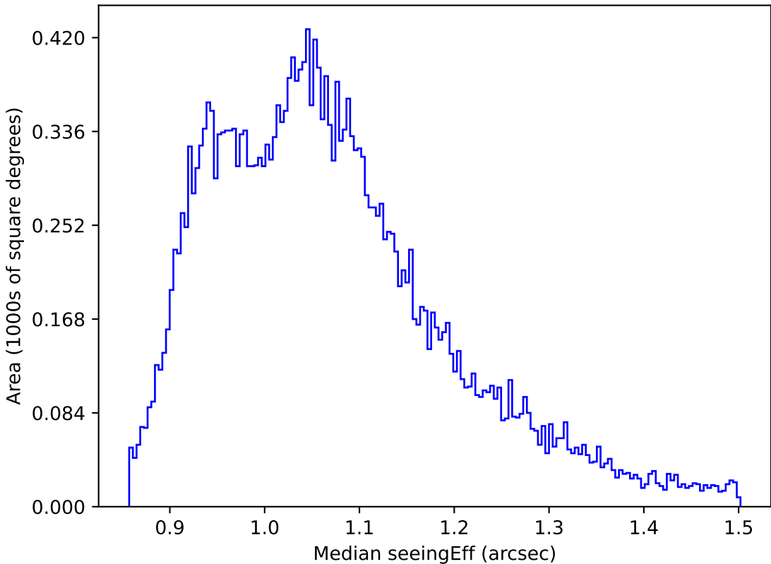
ddf_loaded_half_fl15_v3.4_10yrs All sky r band: Median seeingEff
