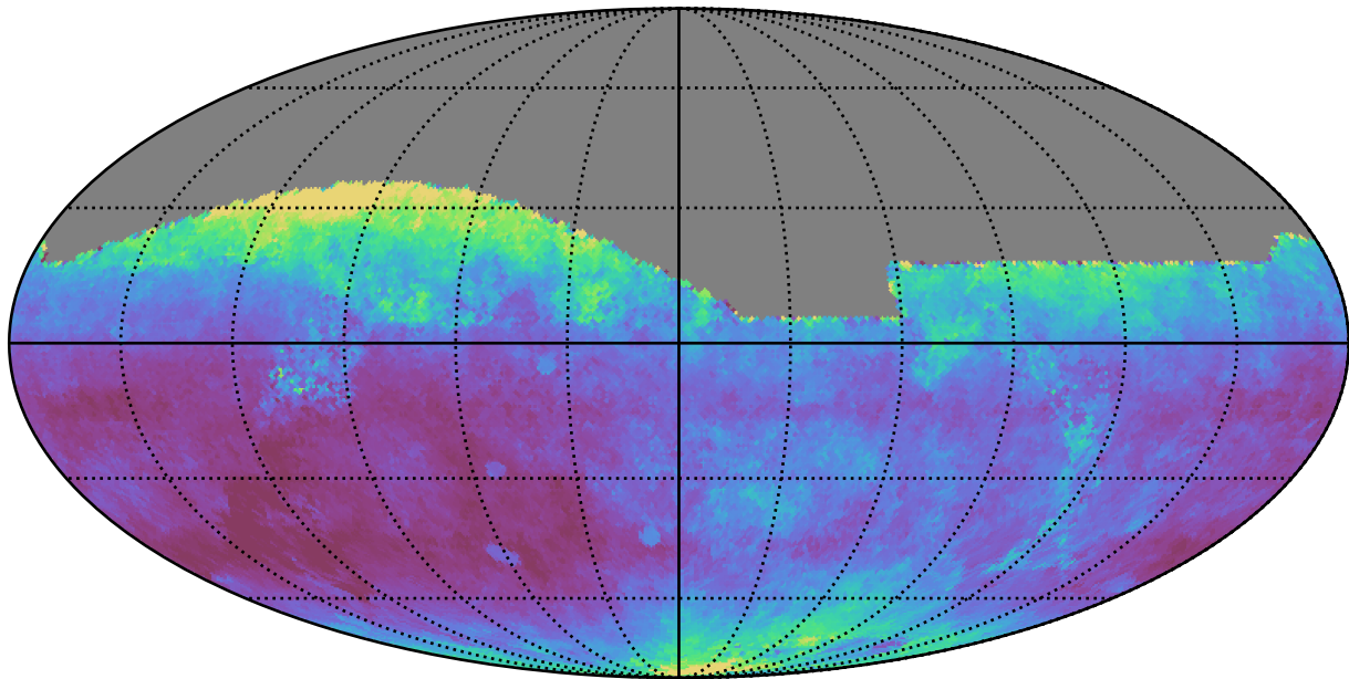
ddf_loaded_half_fl15_v3.4_10yrs All sky i band: Median seeingEff
