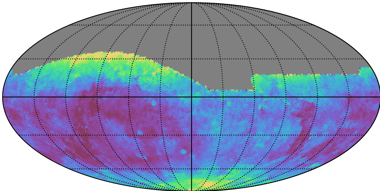
ddf_loaded_half_fl15_v3.4_10yrs All sky g band: Median seeingEff
