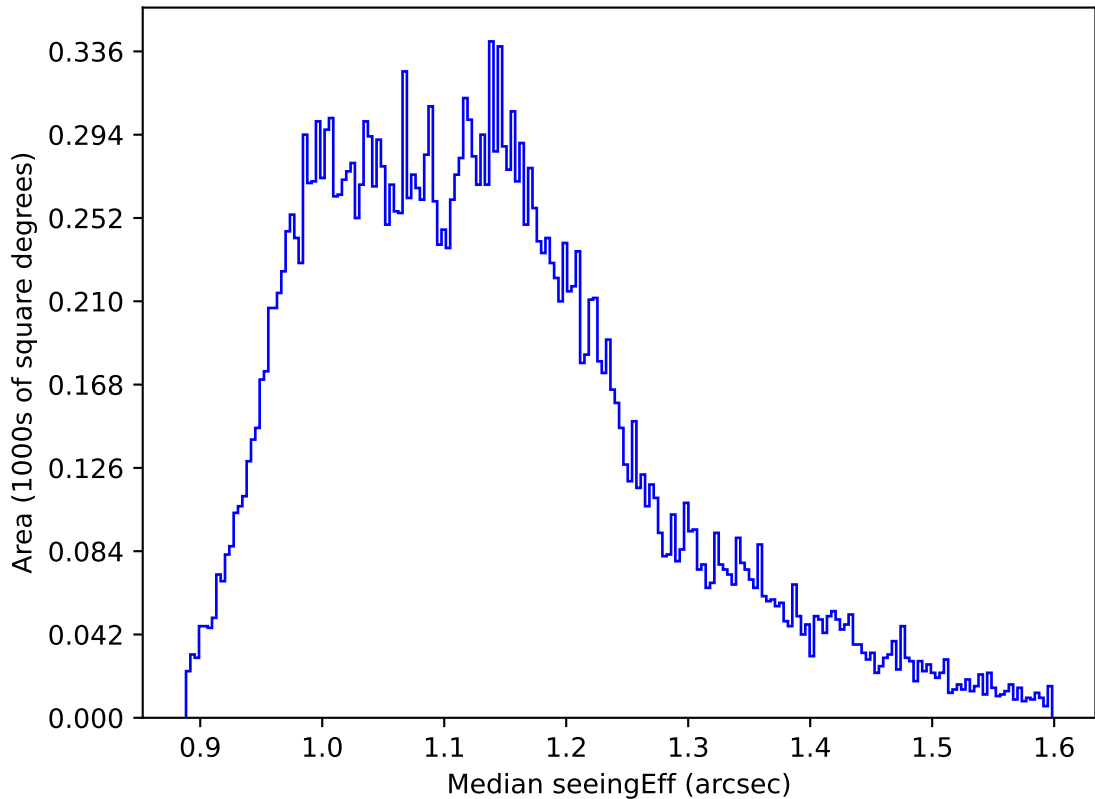
ddf_loaded_half_fl15_v3.4_10yrs All sky g band: Median seeingEff
