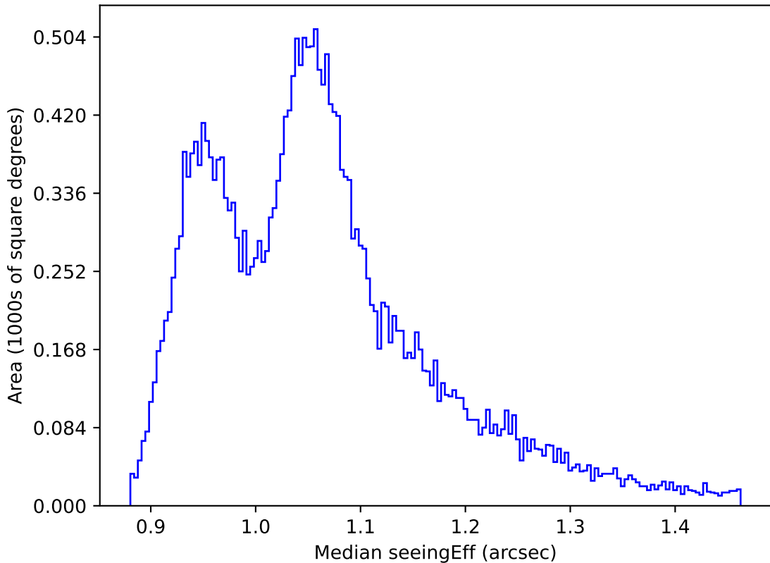
ddf_loaded_half_fl15_v3.4_10yrs All sky all bands: Median seeingEff
