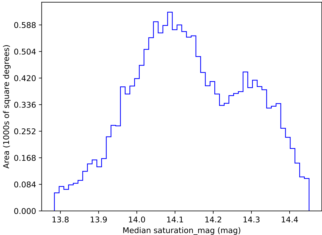
ddf_loaded_half_fl15_v3.4_10yrs WFD z band: Median saturation_mag
