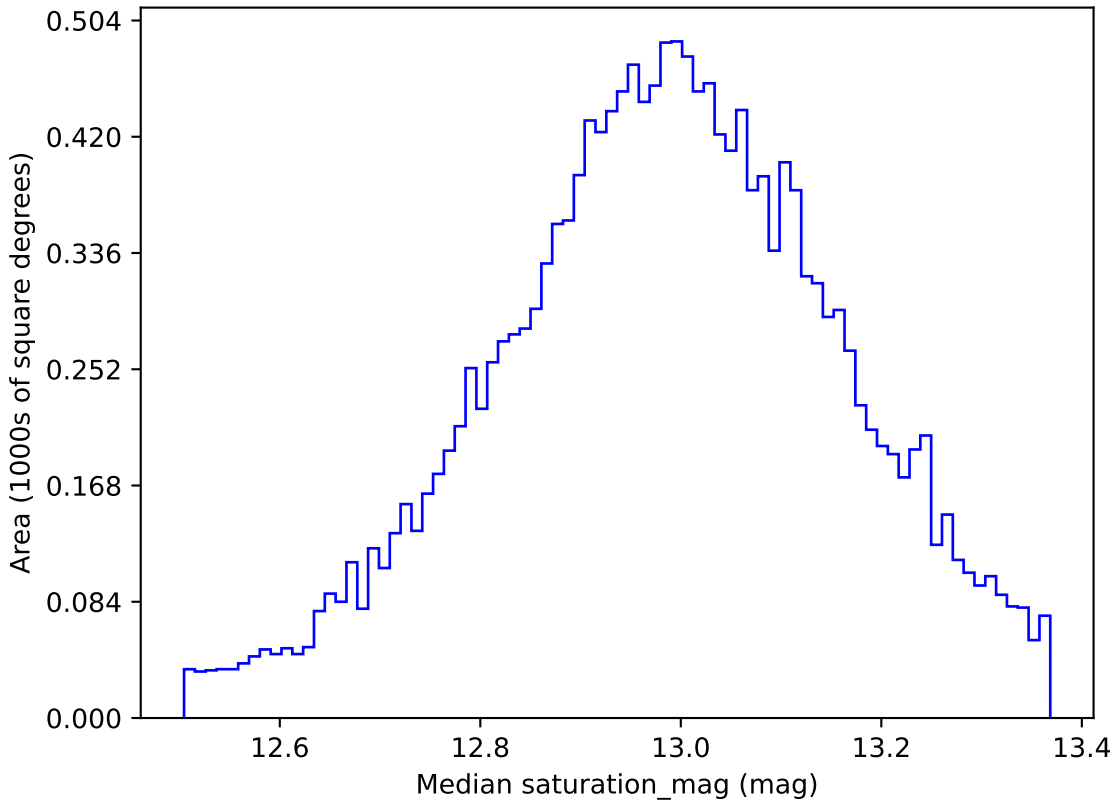
ddf_loaded_half_fl15_v3.4_10yrs WFD u band: Median saturation_mag
