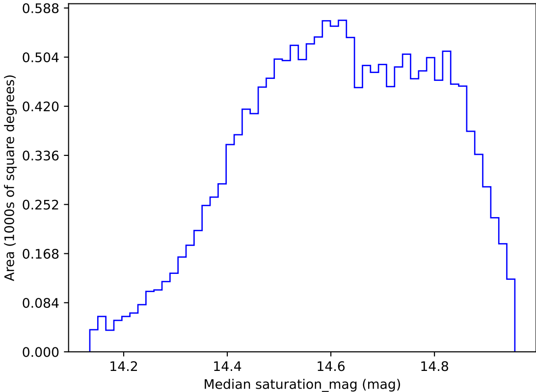
ddf_loaded_half_fl15_v3.4_10yrs WFD r band: Median saturation_mag
