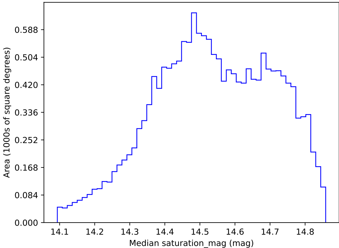
ddf_loaded_half_fl15_v3.4_10yrs WFD i band: Median saturation_mag
