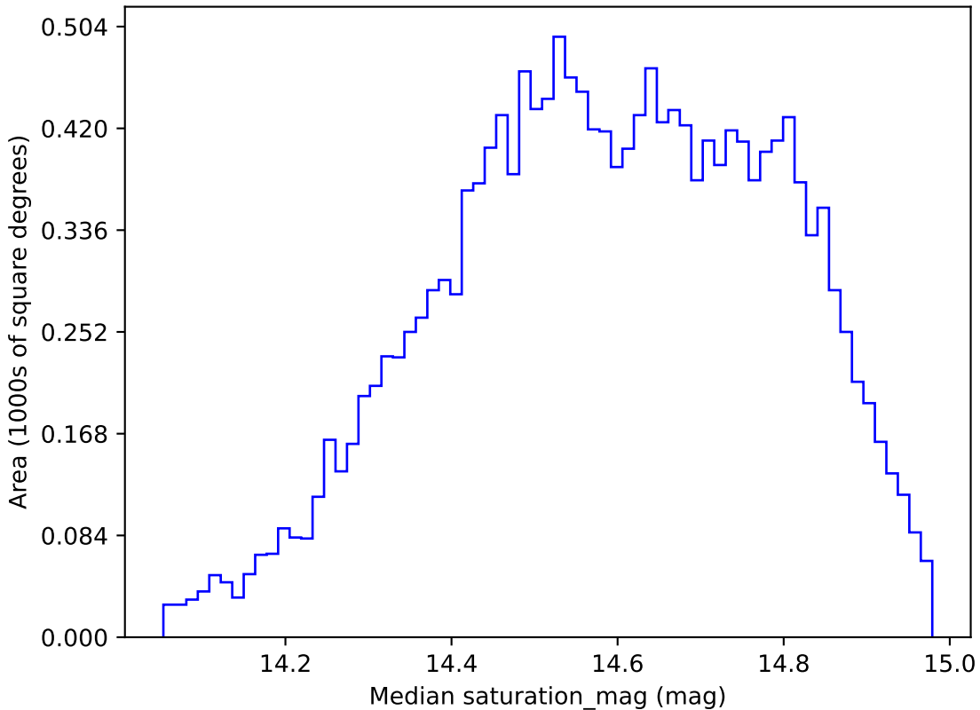
ddf_loaded_half_fl15_v3.4_10yrs WFD g band: Median saturation_mag
