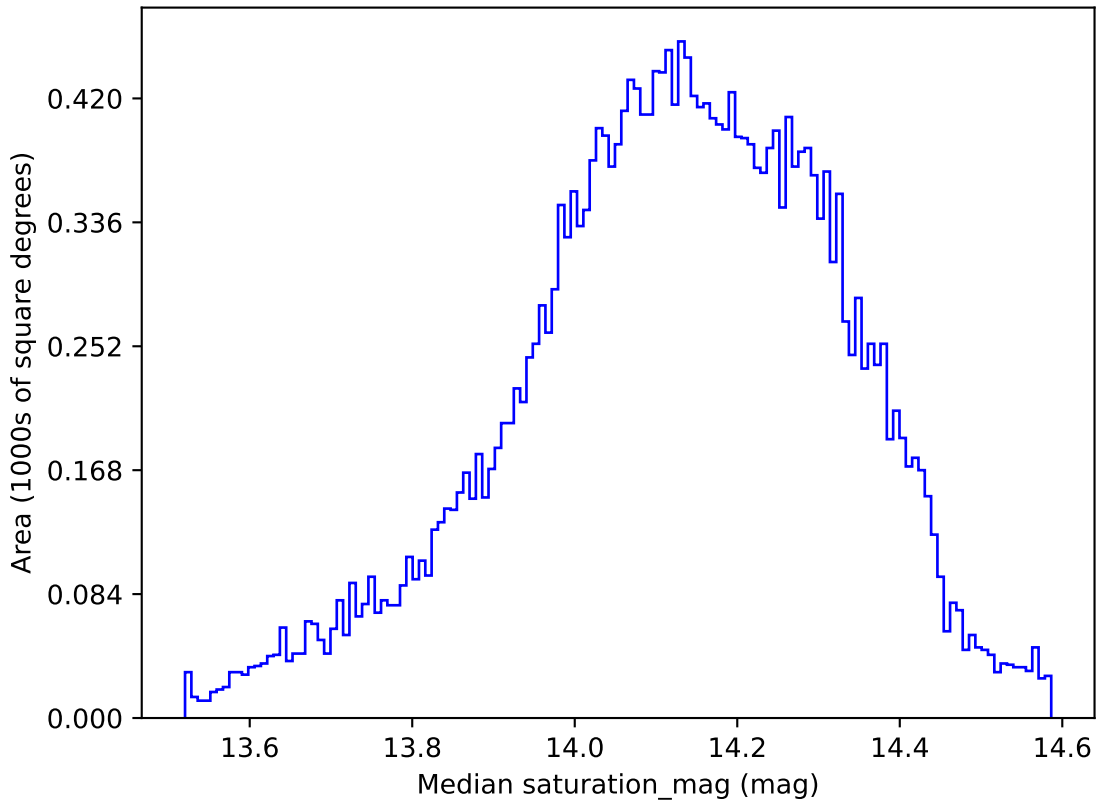
ddf_loaded_half_fl15_v3.4_10yrs All sky all bands: Median saturation_mag
