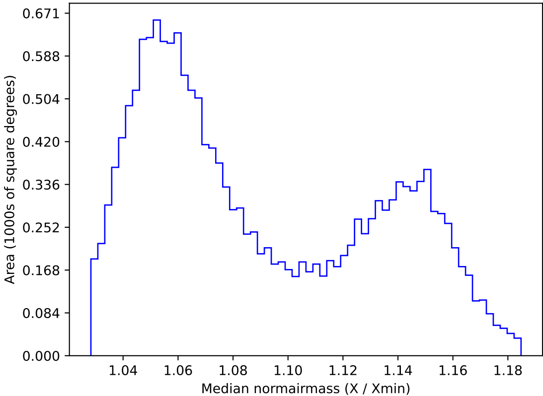
ddf_loaded_half_fl15_v3.4_10yrs WFD y band: Median normairmass
