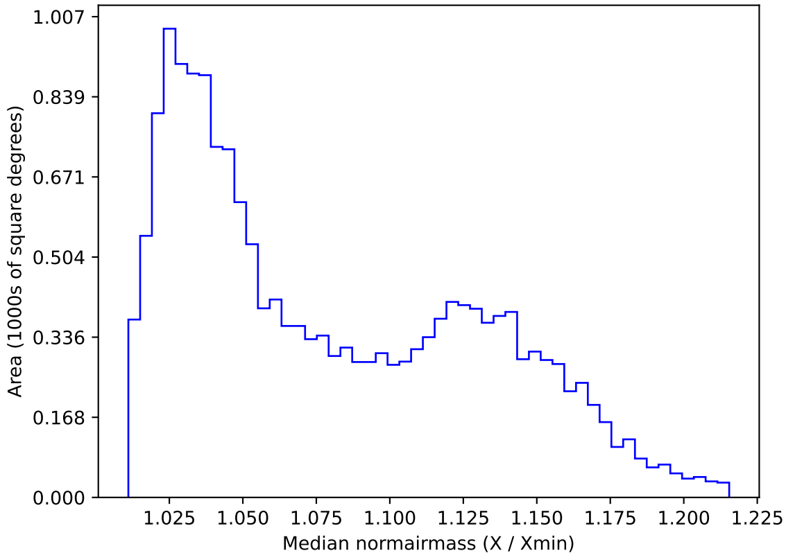
ddf_loaded_half_fl15_v3.4_10yrs WFD u band: Median normairmass
