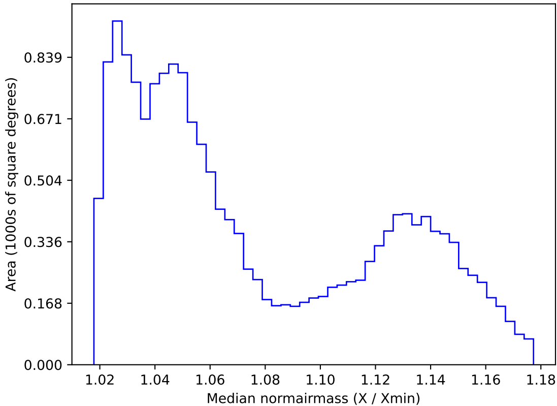
ddf_loaded_half_fl15_v3.4_10yrs WFD r band: Median normairmass
