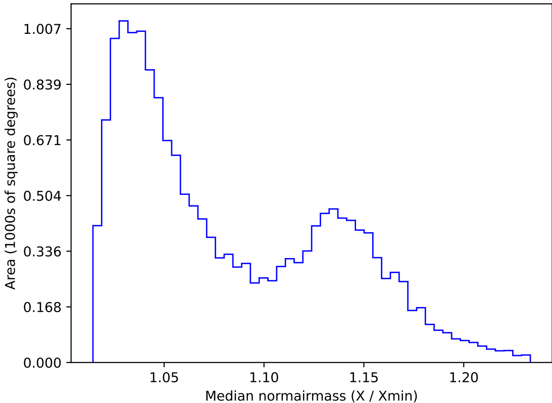
ddf_loaded_half_fl15_v3.4_10yrs WFD g band: Median normairmass
