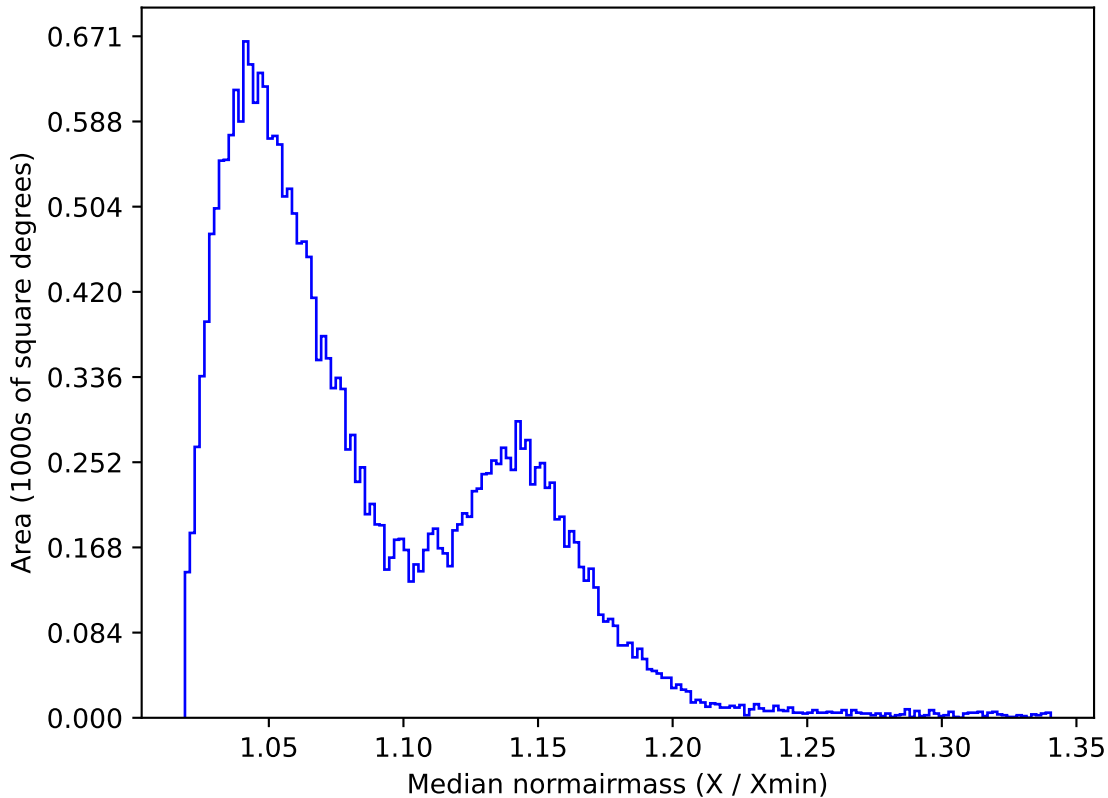
ddf_loaded_half_fl15_v3.4_10yrs All sky z band: Median normairmass
