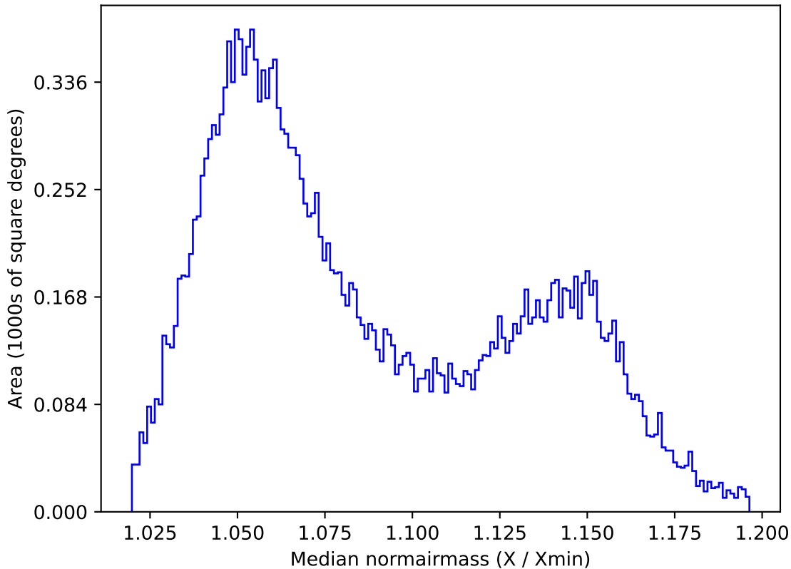
ddf_loaded_half_fl15_v3.4_10yrs All sky y band: Median normairmass
