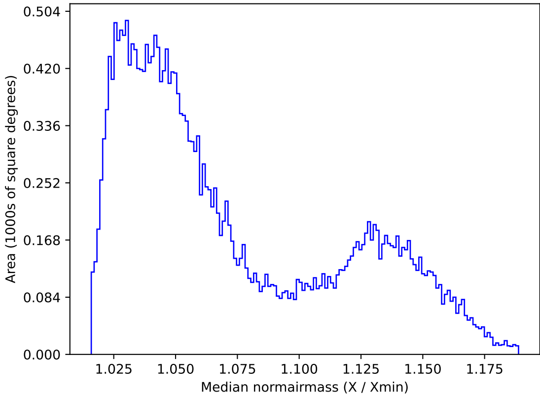
ddf_loaded_half_fl15_v3.4_10yrs All sky r band: Median normairmass
