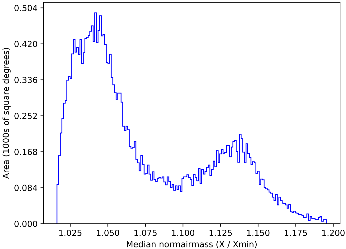
ddf_loaded_half_fl15_v3.4_10yrs All sky i band: Median normairmass
