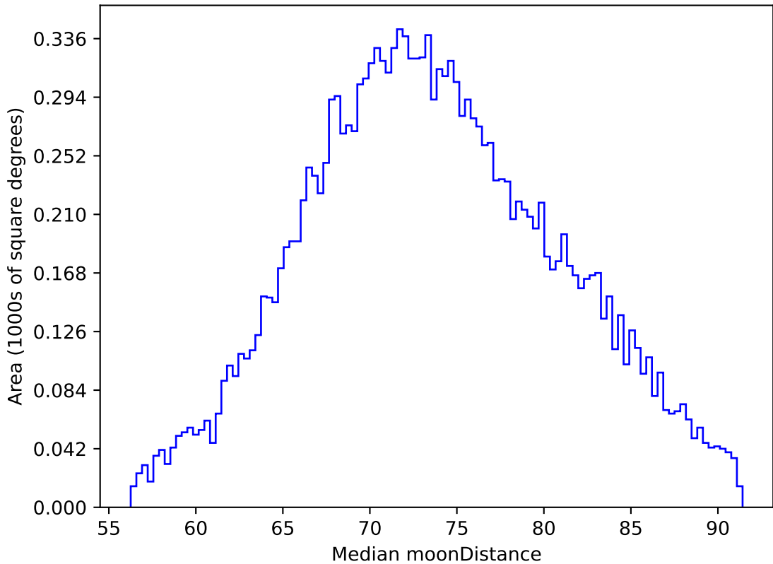
ddf_loaded_half_fl15_v3.4_10yrs WFD z band: Median moonDistance
