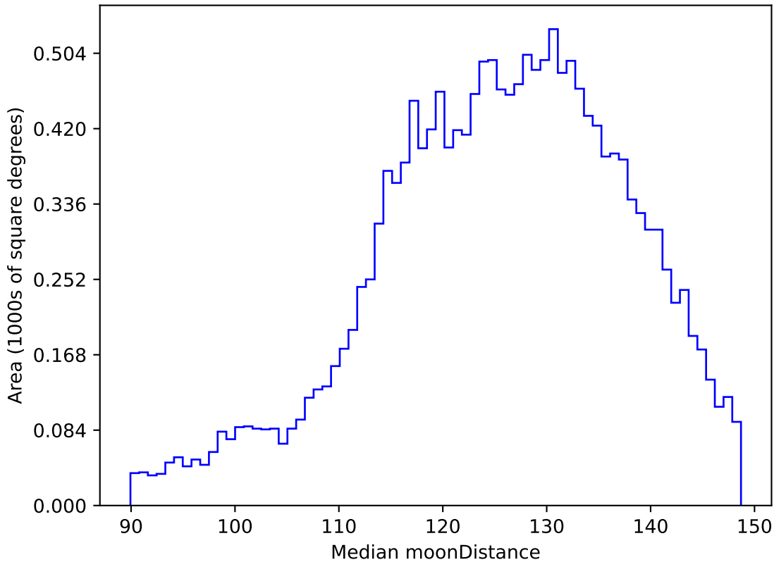
ddf_loaded_half_fl15_v3.4_10yrs WFD u band: Median moonDistance
