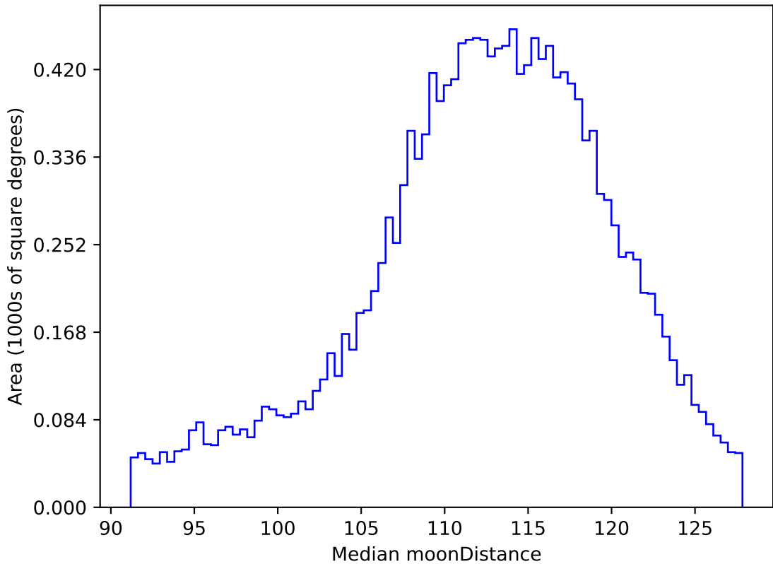
ddf_loaded_half_fl15_v3.4_10yrs WFD r band: Median moonDistance
