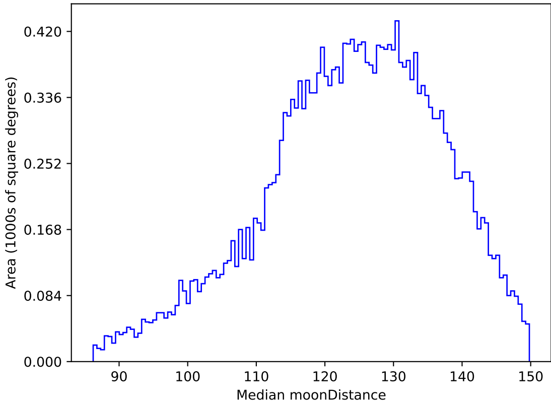
ddf_loaded_half_fl15_v3.4_10yrs All sky u band: Median moonDistance
