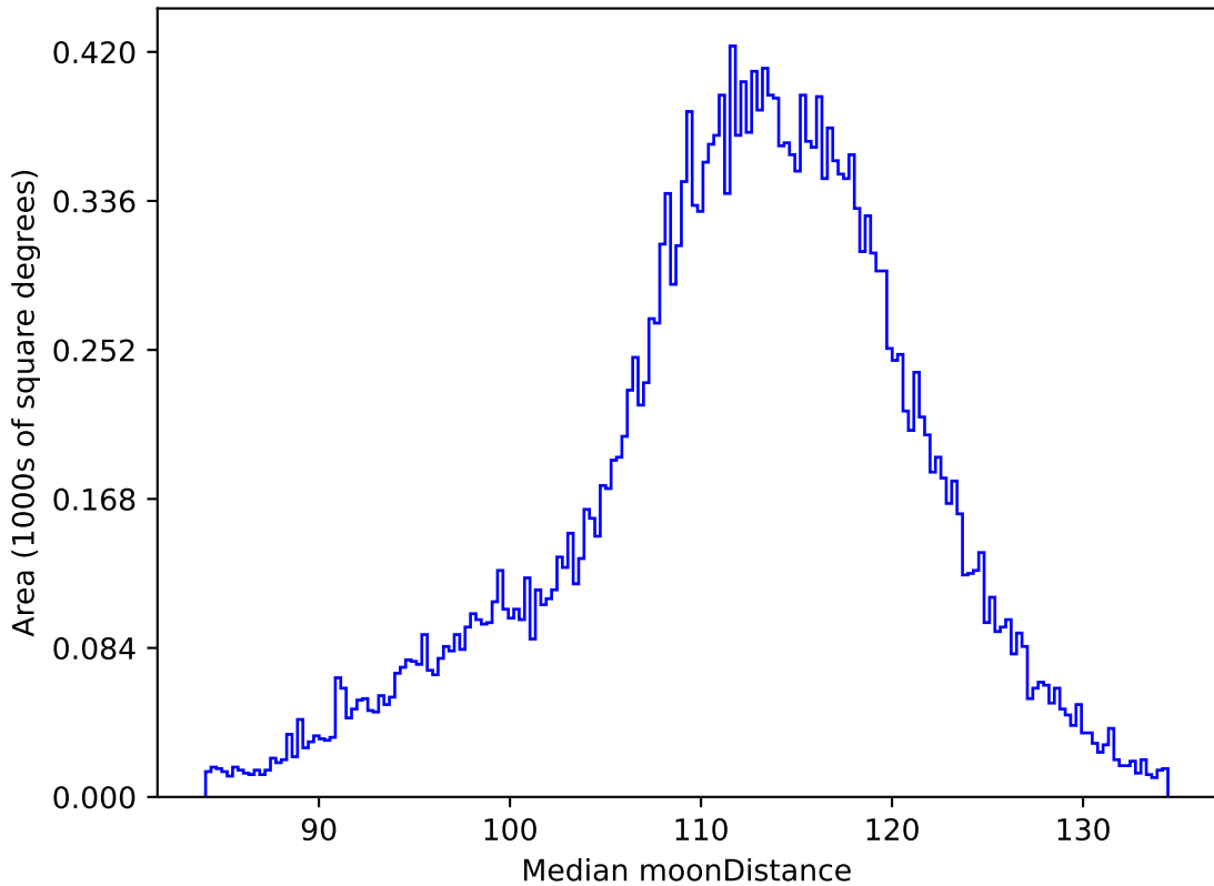
ddf_loaded_half_fl15_v3.4_10yrs All sky r band: Median moonDistance
