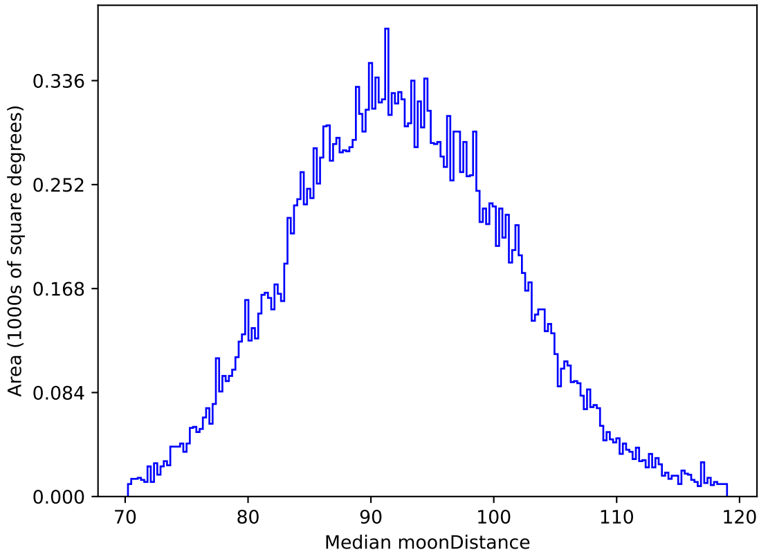
ddf_loaded_half_fl15_v3.4_10yrs All sky i band: Median moonDistance
