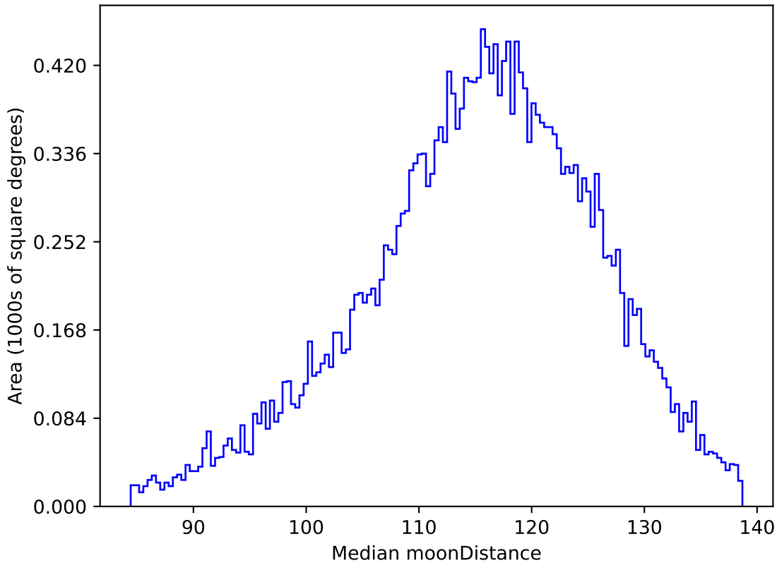
ddf_loaded_half_fl15_v3.4_10yrs All sky g band: Median moonDistance
