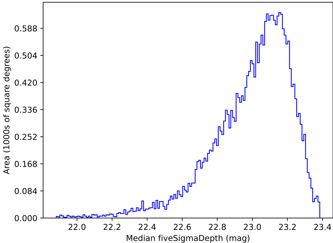
ddf_loaded_half_fl15_v3.4_10yrs Yr 1 z band: Median fiveSigmaDepth
