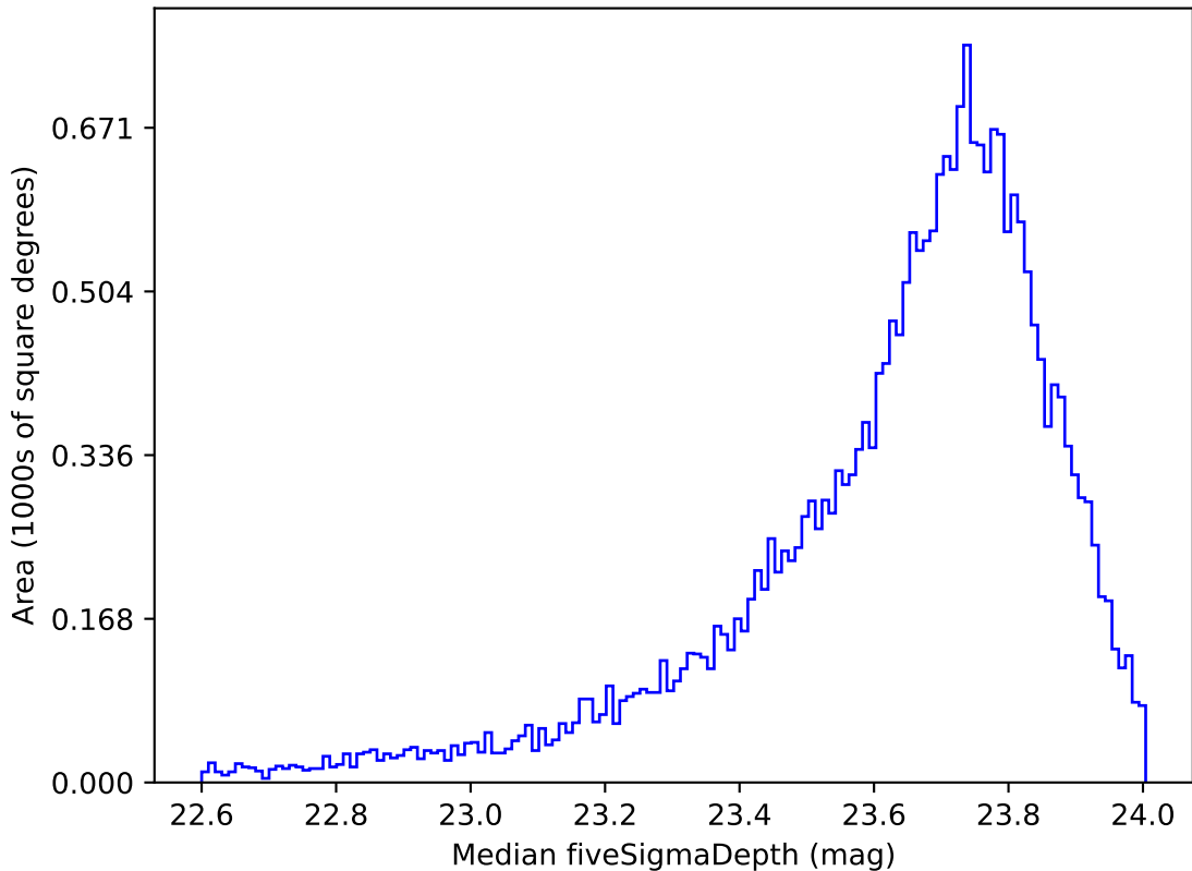
ddf_loaded_half_fl15_v3.4_10yrs Yr 1 i band: Median fiveSigmaDepth
