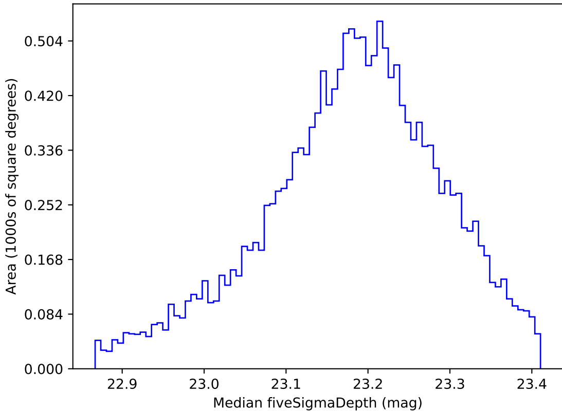
ddf_loaded_half_fl15_v3.4_10yrs WFD u band: Median fiveSigmaDepth
