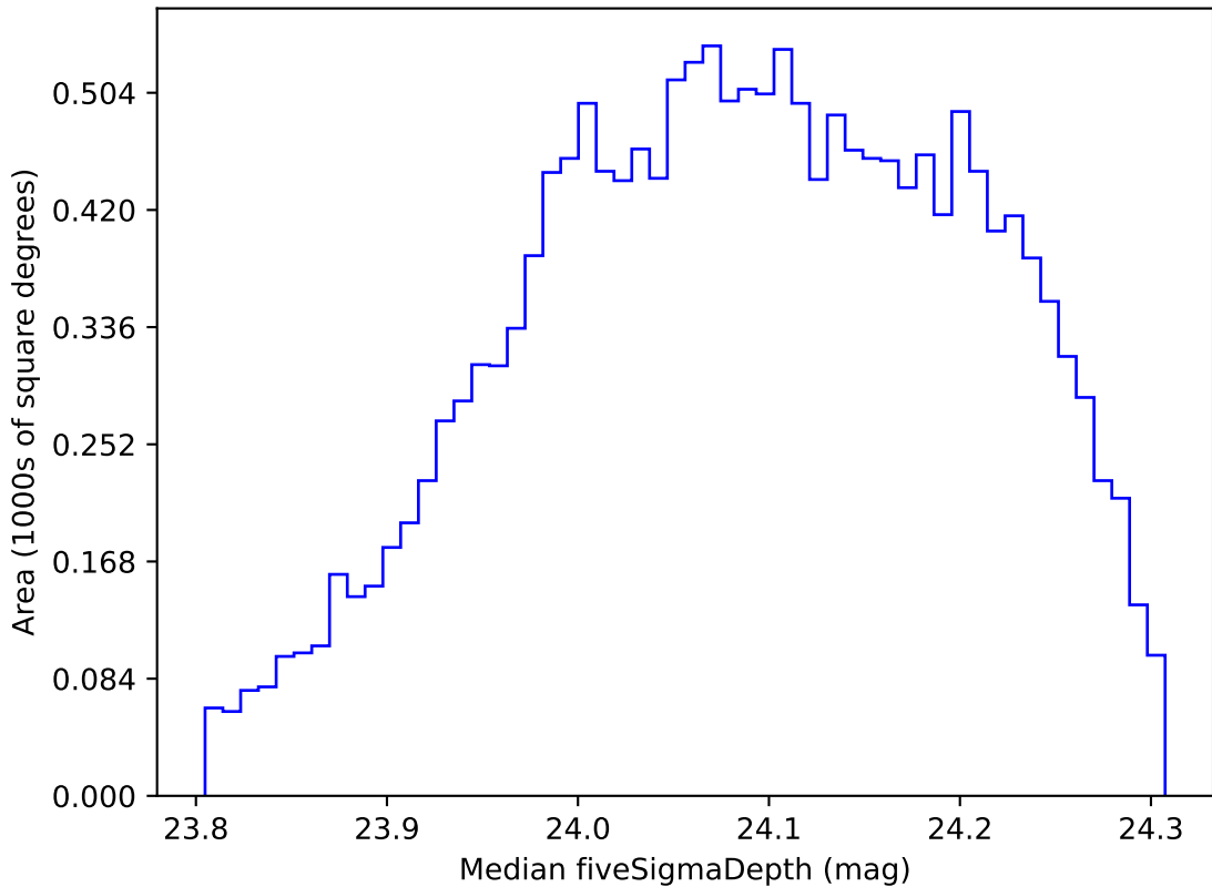
ddf_loaded_half_fl15_v3.4_10yrs WFD r band: Median fiveSigmaDepth
