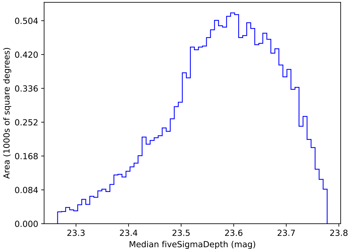
ddf_loaded_half_fl15_v3.4_10yrs WFD i band: Median fiveSigmaDepth
